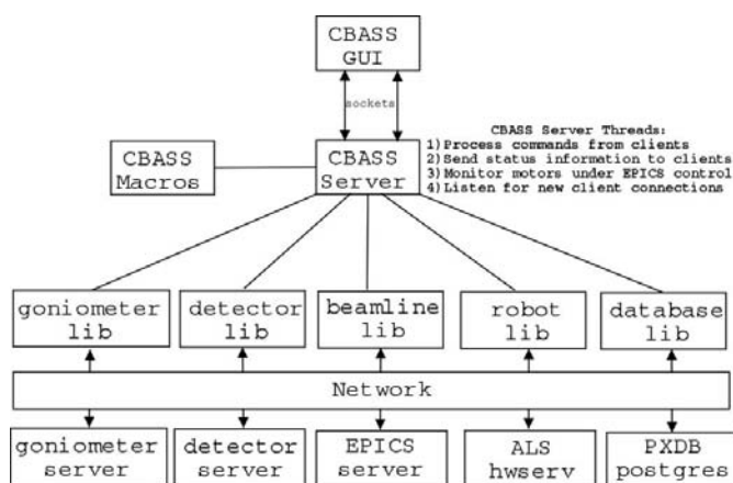
Figure 6 Architecture of CBASS .
